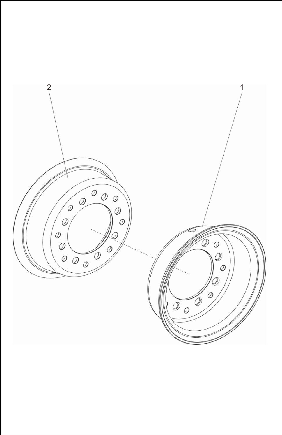
图3-A-1 轮辋总成4.00E-9/轮辋总成5.00F-10 Figure3-A-1 Rim assembly 256715511001/256815511001
