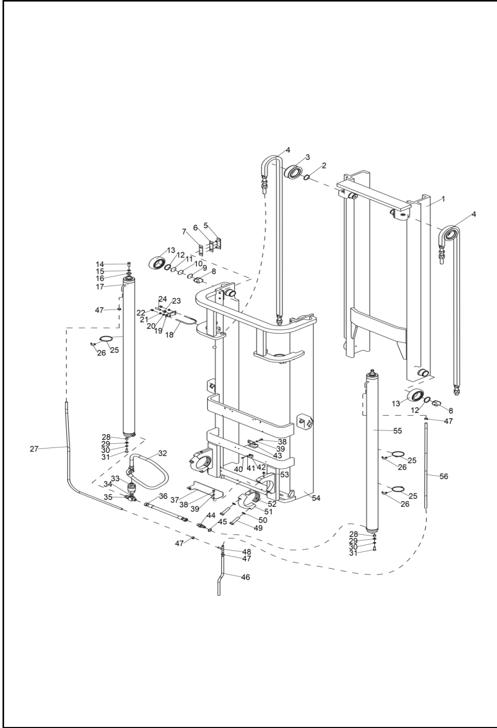
图14-H 门架总成(3.0t) Figure14-H Frame assembly (3.0t) 293344001117 (二级门架通用)
