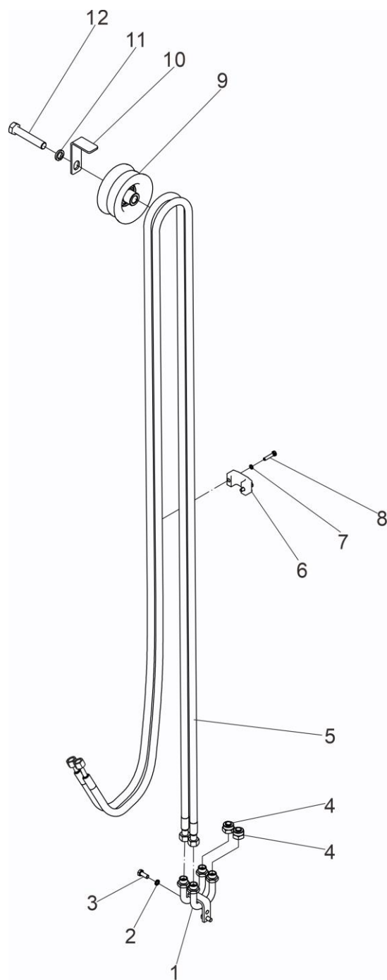
图14-F 属具管路总成(二级门架单附加) (3.5/3.8t) Figure14-F Fittings pipe assembly (Secondary gantry single attached) (3.5/3.8t) 293327501119(20-34)
