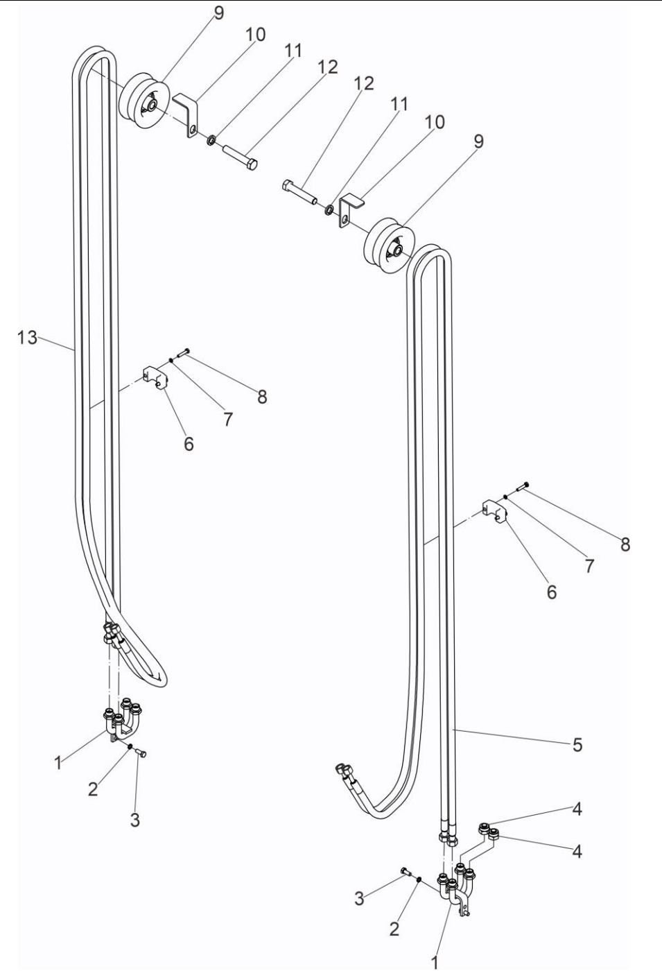
图14-D 属具管路总成(二级门架双附加) (3. 5/3. 8t) Figure14-D Fittings pipe assembly (secondary gantry double attached) (3. 5/3. 8t) 293327501101, 293327501150 (51-64)
